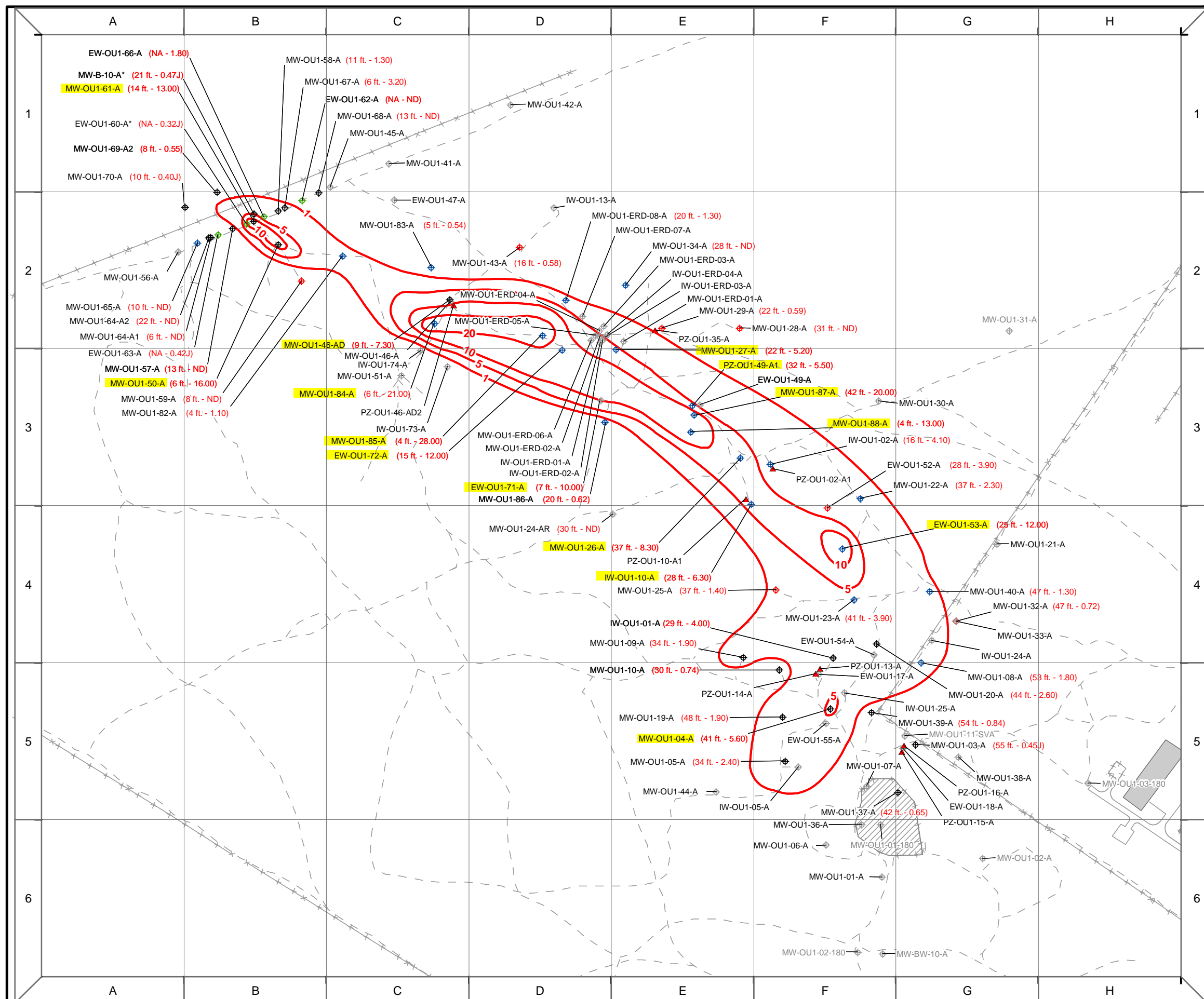
Figure 1.2 OU-1 TCE Concentrations in Groundwater September 2007
